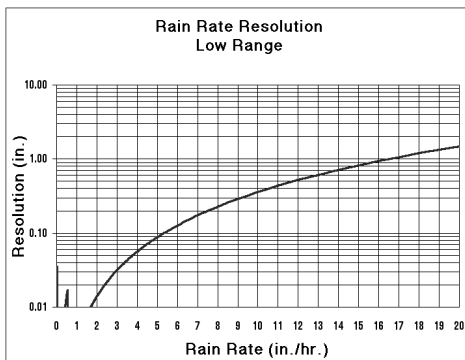
Figure 3. Low Range Rain Rate Resolution
