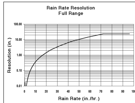
Figure 4. Full Range Rain Rate Resolution
